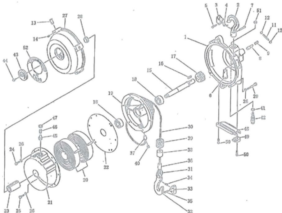
□Parts List for EWF-60, EWF-70
